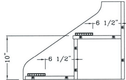
SIDE SECTION
