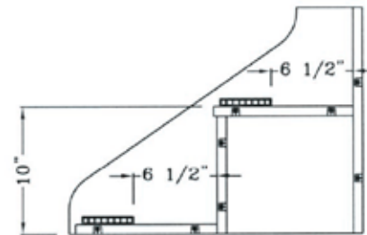
SIDE SECTION
