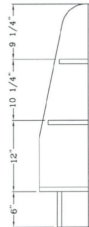
SIDE SECTION
